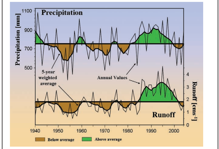
Figure 1. Year-to-year and persistent variations of annual precipitation (top) and annual runoff in the Fort Cobb watershed (bottom).
